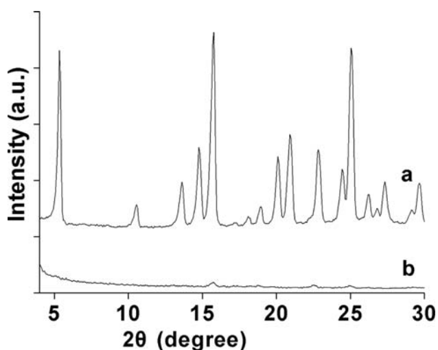
FIGURE 6 XRD Pattern of Commercial ATRA Powder (a) ATRA-NPs (b).
